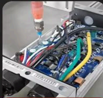
Power adapter potting
